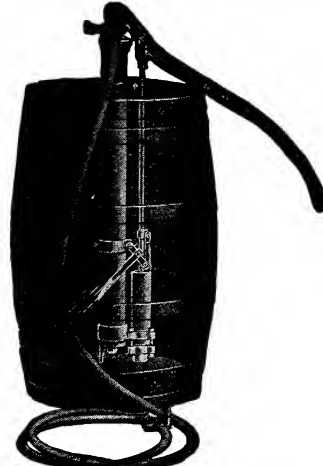
Century Barrel Spray Pump
